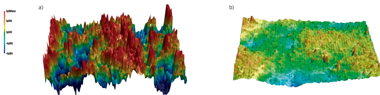
Figure 3: Surface profiles of SLS parts made of L&V TPU LUVOSINT X92A-1: a) without surface treatment, b) with VFS surface treatment. All images are stretched by factor 5 in the z-direction to better illustrate the differences in roughness.
